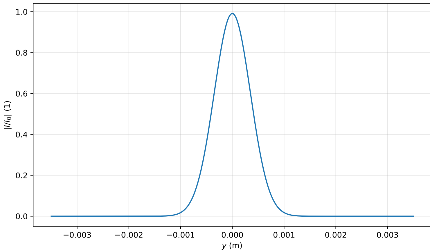
Intensity profile I(x=0, y, z=0.239)/I_0 , P_{in}=0.1P_{cr} , artificial time
